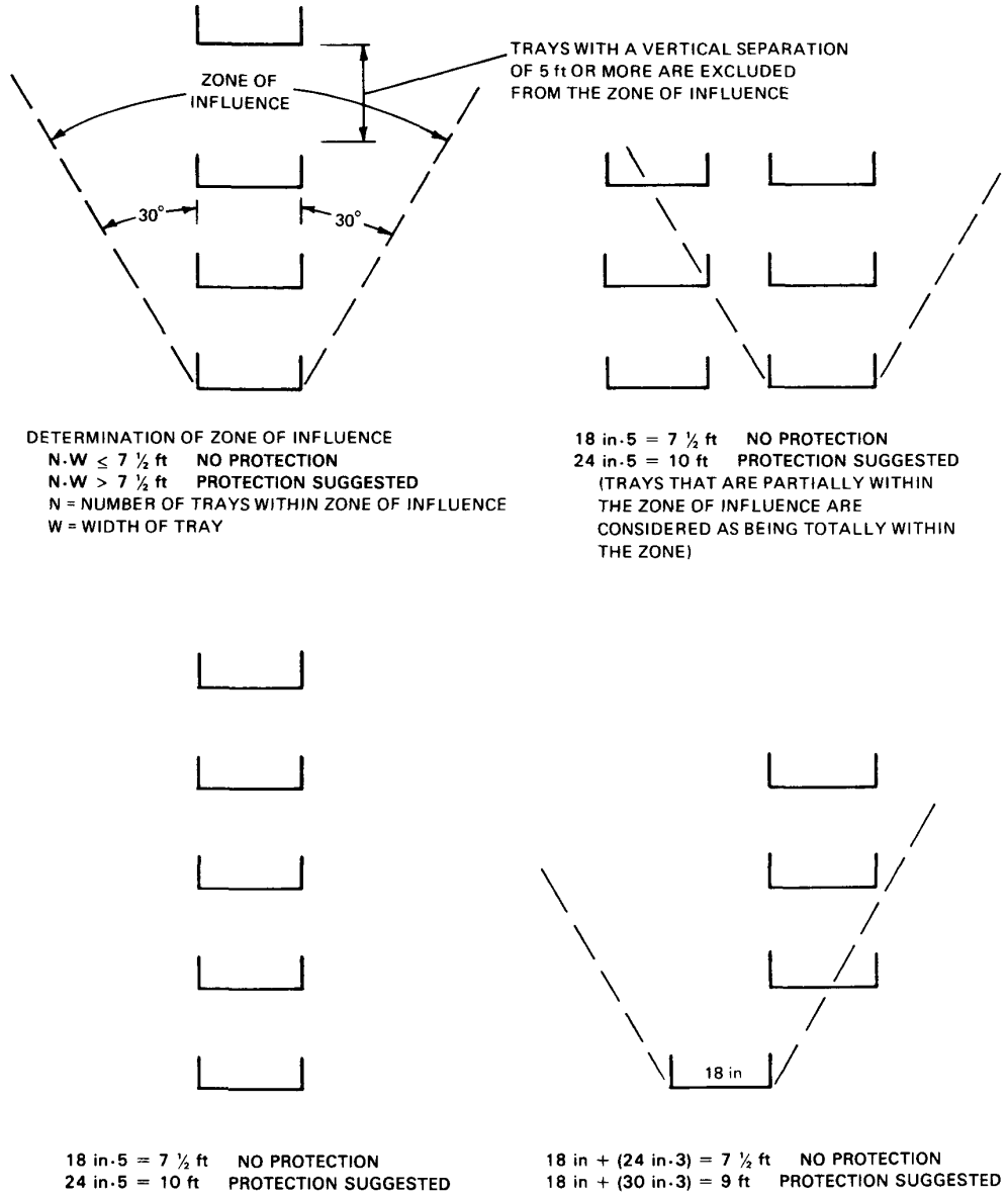
Fig 1 Determination of Potential High Cable Concentration
